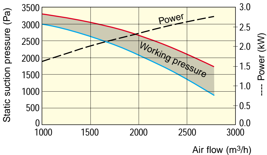
Suction pressure
